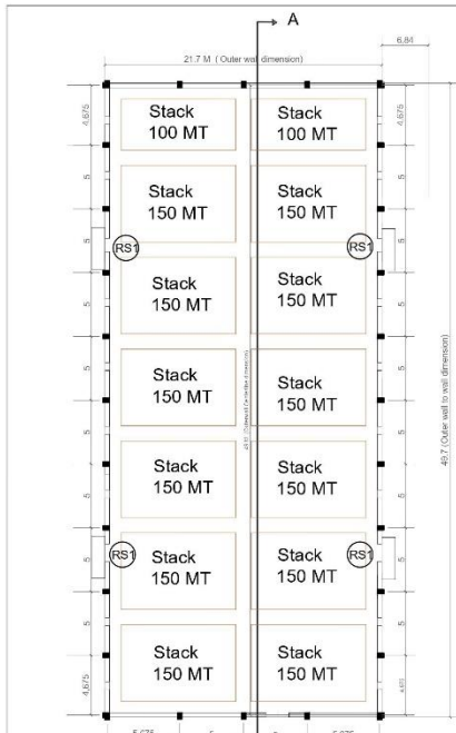
WAREHOUSE PLAN WITH STACK.
