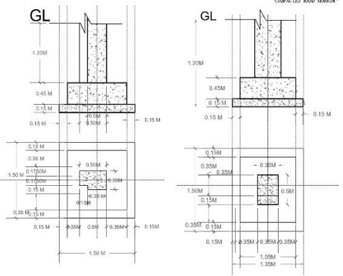
C1 COLUMN FOOTING.
