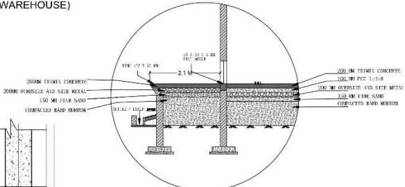
CROSS SECTION PLATFORM. Detail @A
