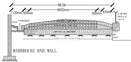
WAREHOUSE END WALL. TYPE CROSS SECTION OF ROAD, APPRON, GUTTER/ DRAIN, WIRE FENCING COMPOUND
